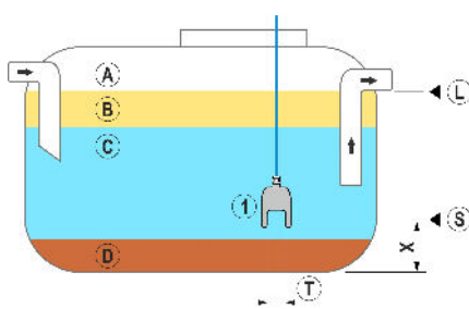
Figure 11. Installing the idOil-SLU sludge sensor
