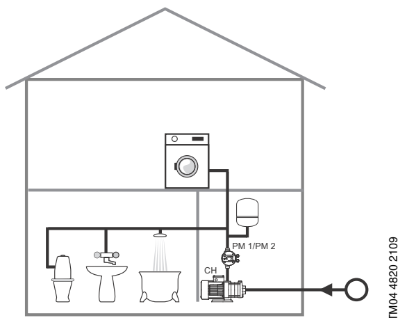
Fig. 7 Boosting of mains water pressure – only allowed in some countries
