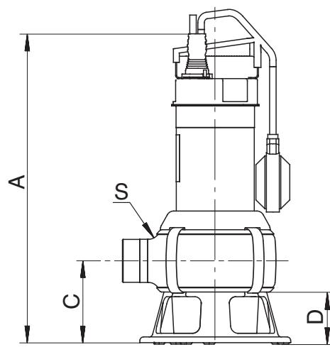
Fig. 36 Pump dimensions
