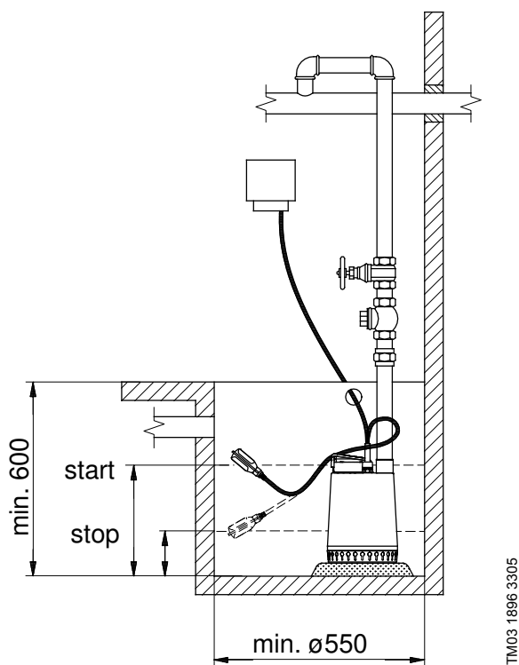
Fig. 16 One-pump installation with float switch
