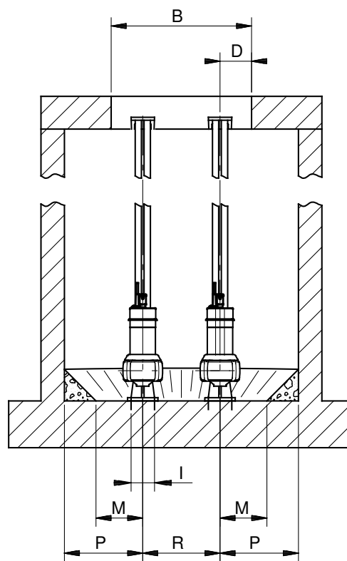
Fig. 39 Dimensional sketch, two-pump installation on auto-coupling system
