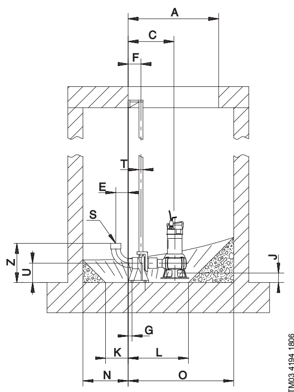
Fig. 38 Dimensional sketch, one-pump installation on auto-coupling system
