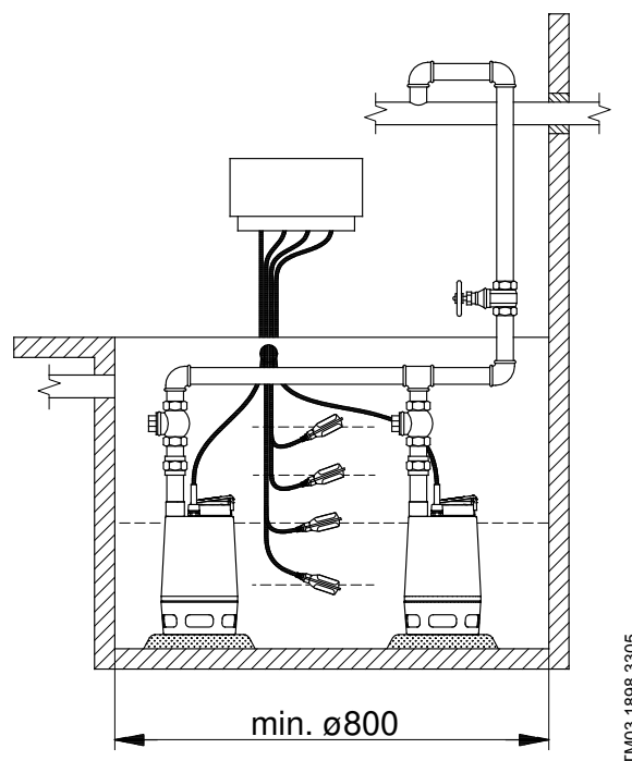
Fig. 33 Two-pump installation with four float switches
