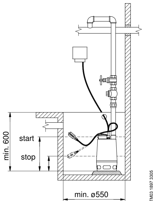
Fig. 32 One-pump installation with float switch
