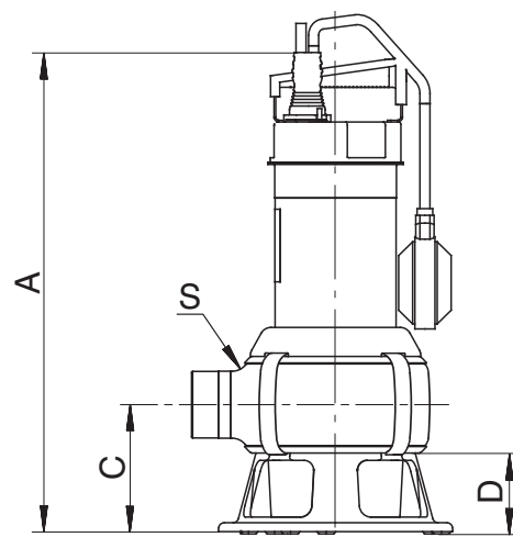
Fig. 25 Pump dimensions
