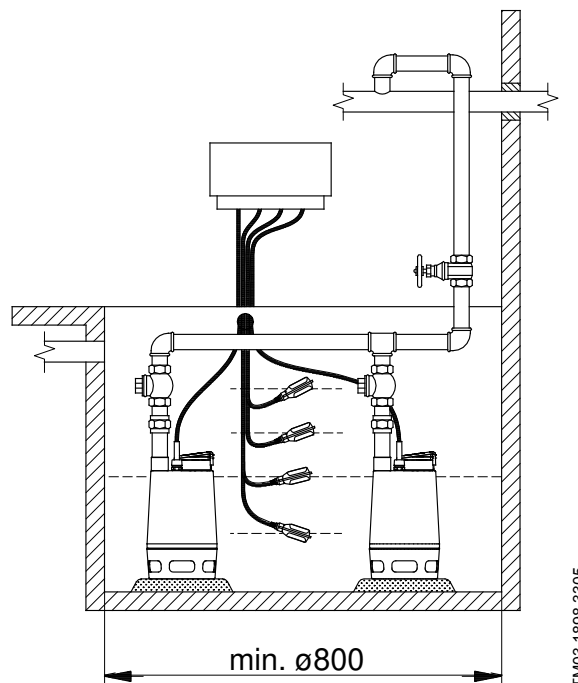
Fig. 22 Two-pump installation with four float switches
