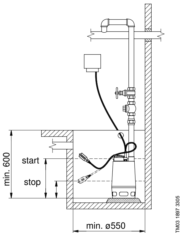
Fig. 21 One-pump installation with float switch
