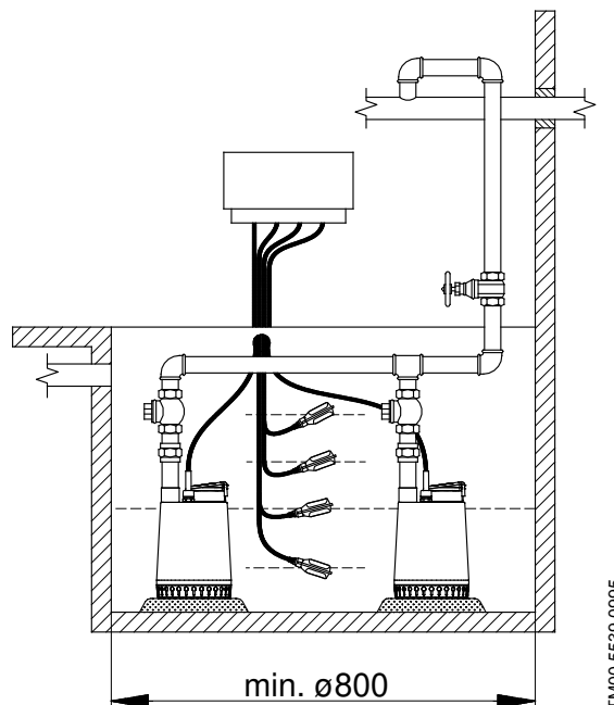
Fig. 17 Two-pump installation with four float switches
