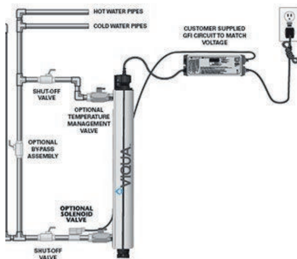
Installationskiss
